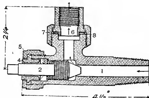
Fig. 3115. Section. TANK-VALVE.
